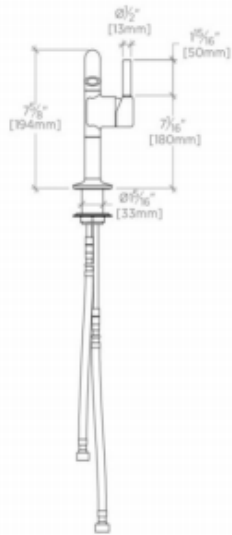
FRONT VIEW
