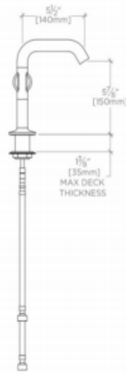
HANDLE OPERATION
