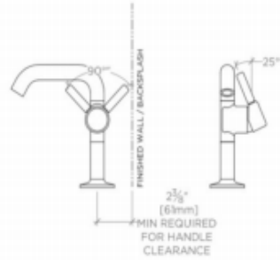
HANDLE OPERATION
