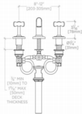
FRONT VIEW SCALE: 3/4"=1'-0"
