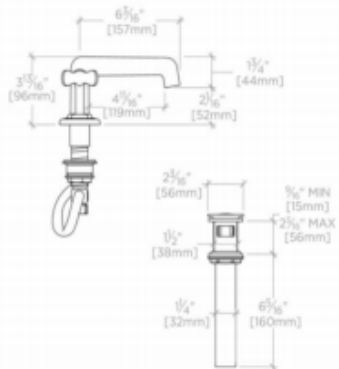
SIDE VIEW SCALE: 3/4"=1'-0"
